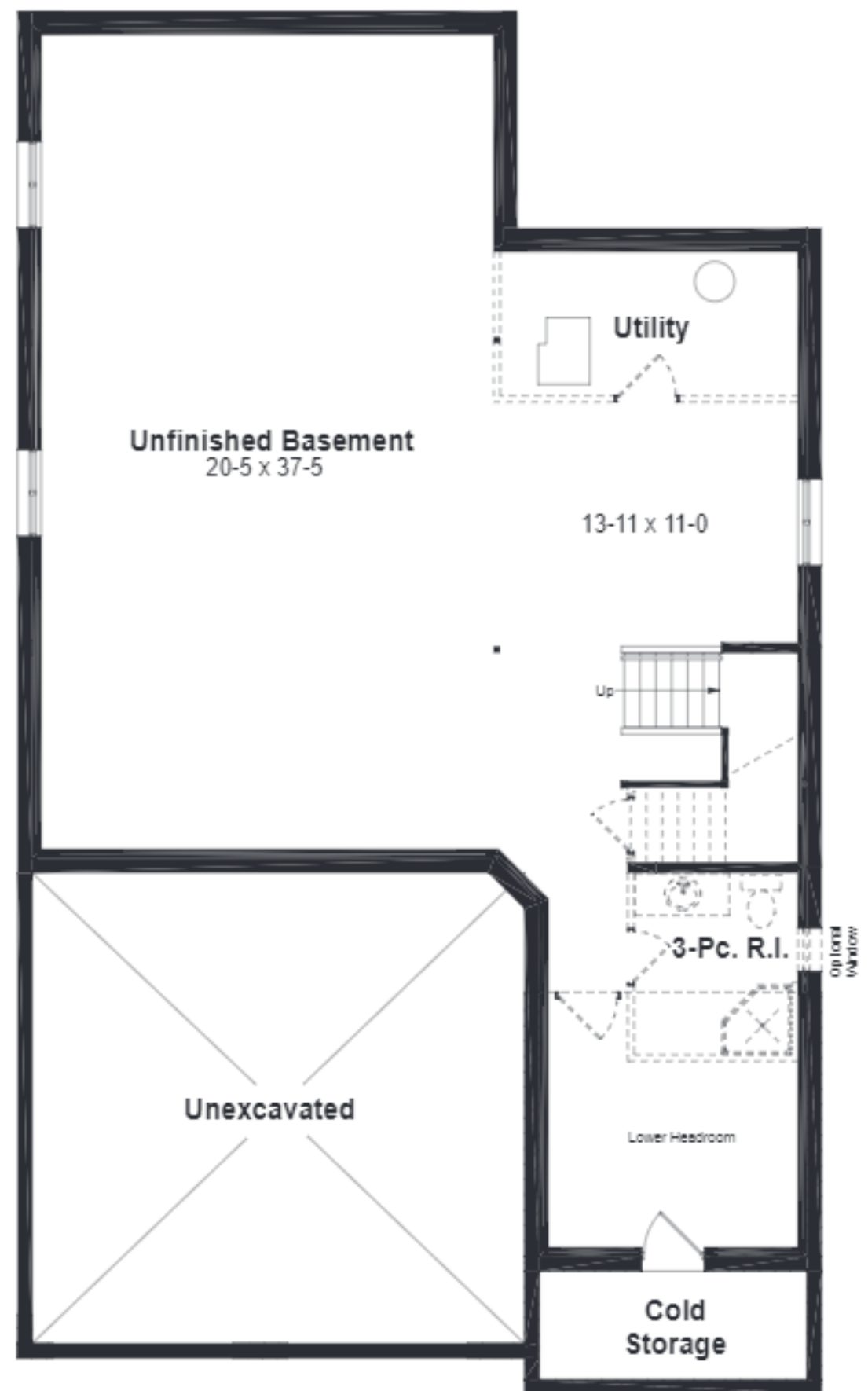
BASEMENT PLAN
