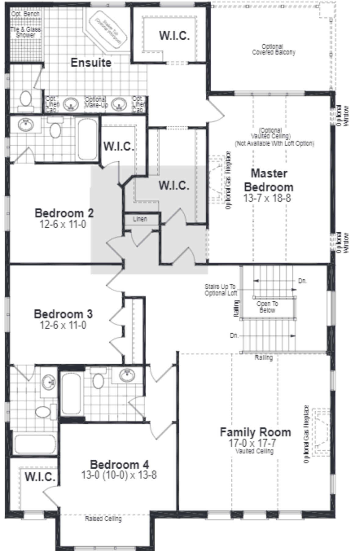
SECOND FLOOR ELEV. 'B'
