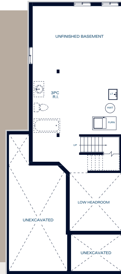
BASEMENT FLOOR PLAN (ELEVATIONS A & B-EWF4516)
